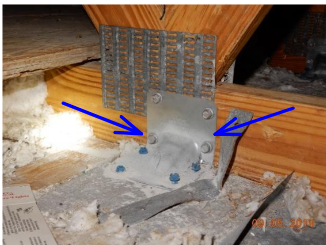
#23 Additional Retrofit Clips with 4 Screws
